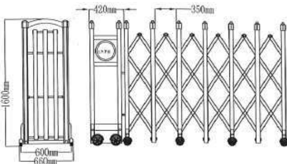
Double Motor for Longer Gates with Heavy Duty Carbon Steel Gear
